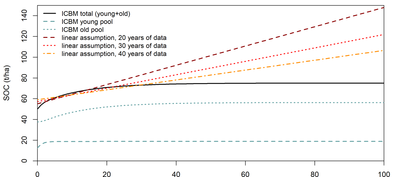
Figure 1: The difference between average sequestration rates (line) and a first-order model (the exponential curve)
