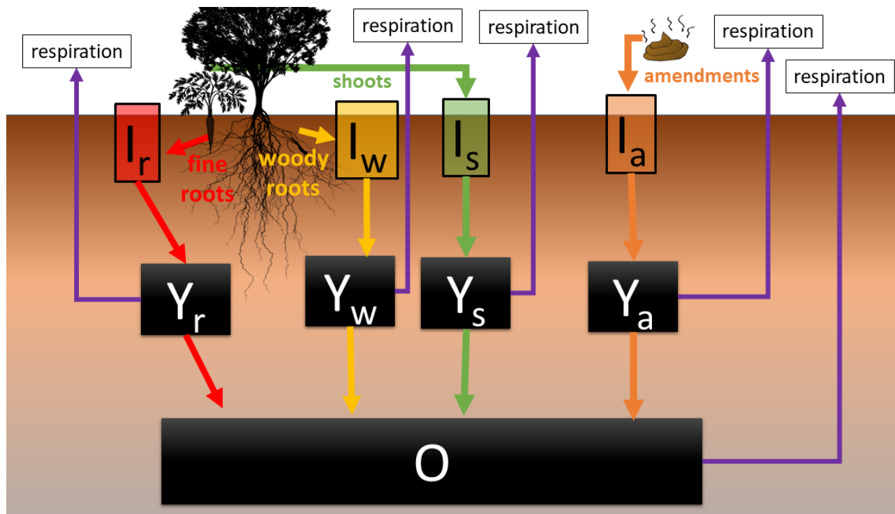
The ICBMagro model structure representing the mass fluxes between the model components. Letters r, w, s and a represent the different input classes (roots, woody root, shoots and amendments, respectively), while the capital letters represent the different pools (I for inputs, Y for the young pools and O for the old pool).
